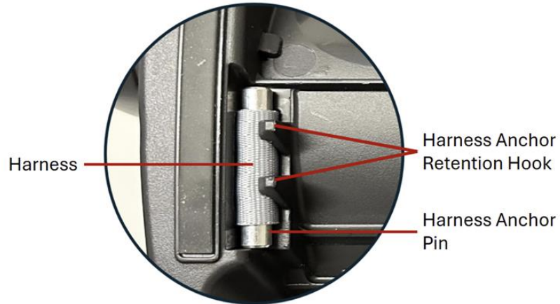
UNDEFORMED HARNESS ANCHOR RETENTION HOOK
